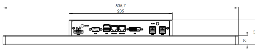
BOTTOM VIEW
